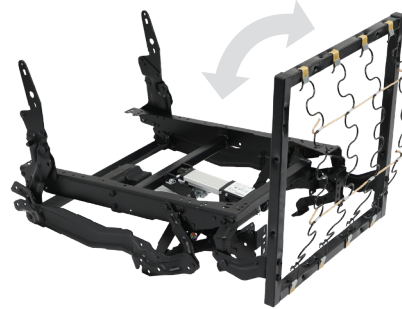
3508 Two-Motor Mechanism
